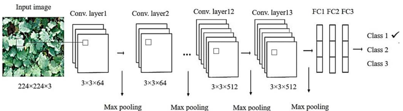
Figure 4. Architecture of Vgg16 for classification of damaged rapeseed crop.
